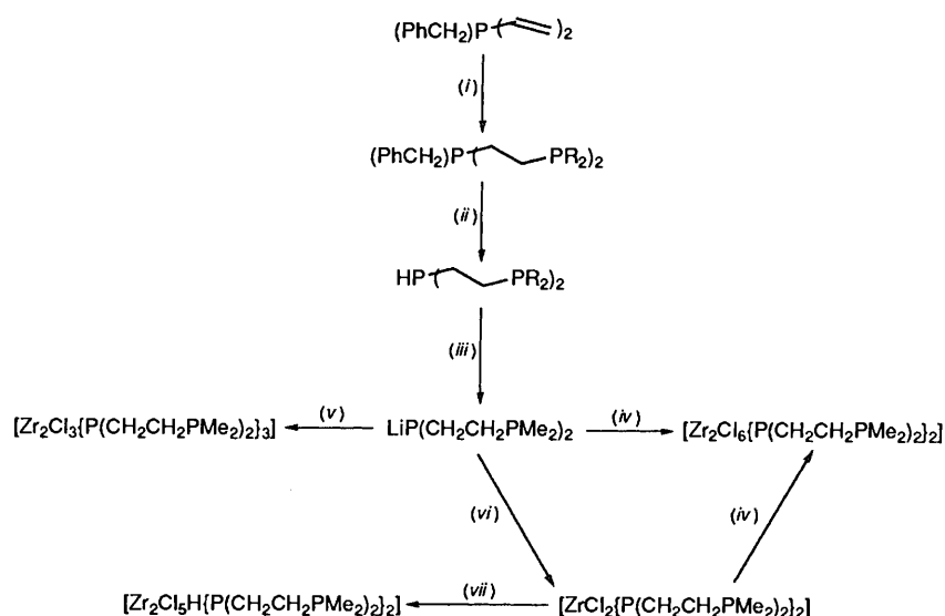
Scheme 1 (i) 2 PR 2 H (R = Me or Et); (ii) Na; (iii) LiBu; (iv) ZrCl 4 ; (v) \frac{1}{3} ZrCl 4 ; (vi) \frac{1}{2} ZrCl 4 ; (vii) MBPh 4 (M = Na or Ag)
